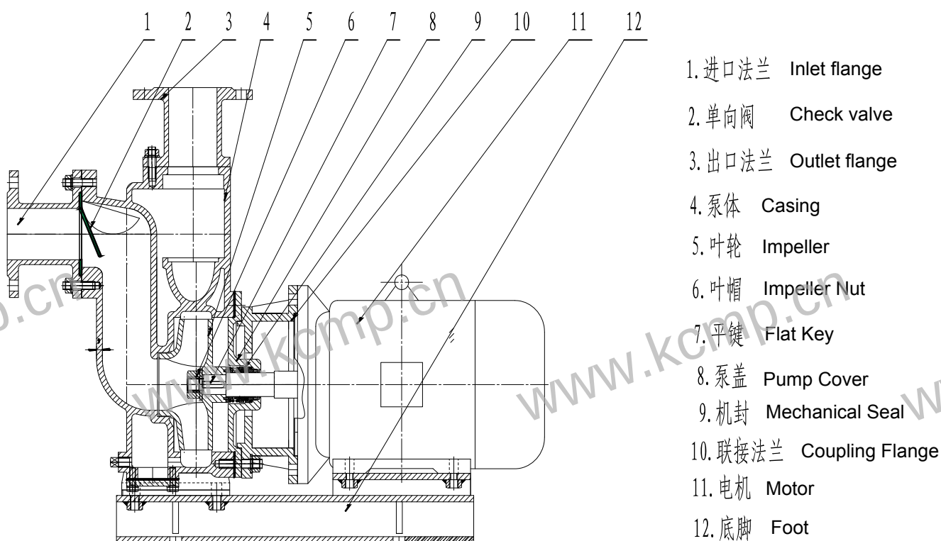
泵的结构图 Structure of pump drawing
