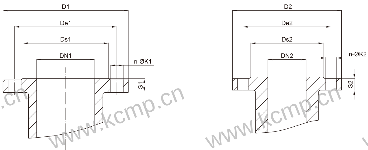
泵吸入口、排出口法兰 Inlet & outlet flange of pump.
